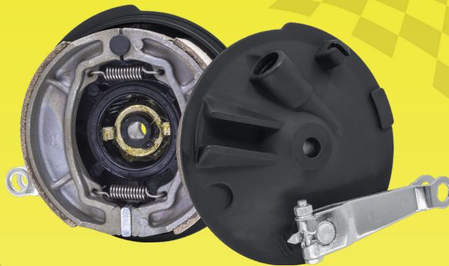
REM2589 Porta balata delantero FT 125 2009-2016, FT 150TS 2016- 2020, DT125 2017-2019 (RIN ASPAS)
